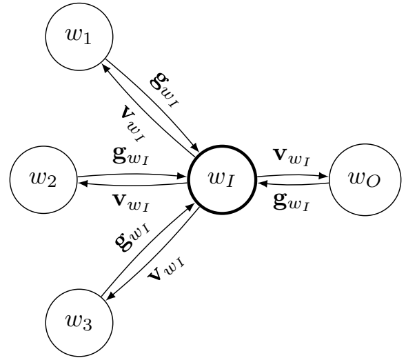
Figure 1: Baseline Negative Sampling Communication Pattern during processing of skip-gram (w_I, w_O) , for 3 negative samples w_1, w_2, w_3 .
