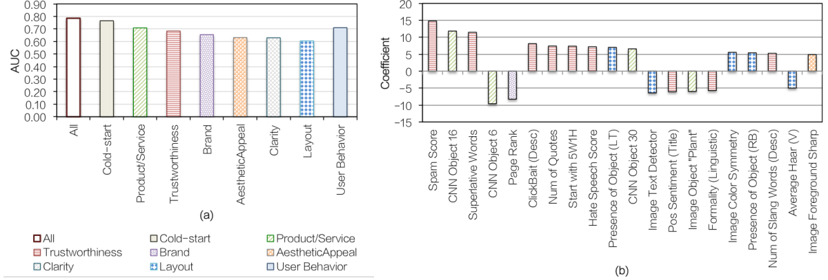
Figure 4: Predicting Pre-click Ad Quality: (a) Feature Subset; (b) Top Significant Feature Coefficients.
