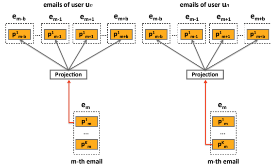
Figure 3: bagged-prod2vec model updates
