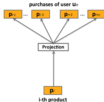
Figure 2: prod2vec skip-gram model
